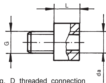
Fig. D threaded connection
